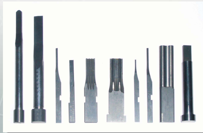
Various Round Punches, TiCN Coating, with Air Hole, Straight Type, Short Type, Two Step Type, with Key Groove, Block Punches.
